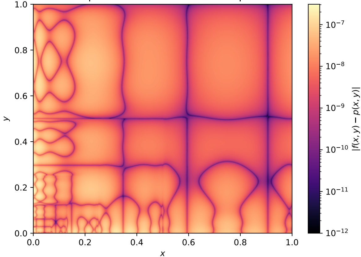
Absolute interpolation error for Genz corner peak function
